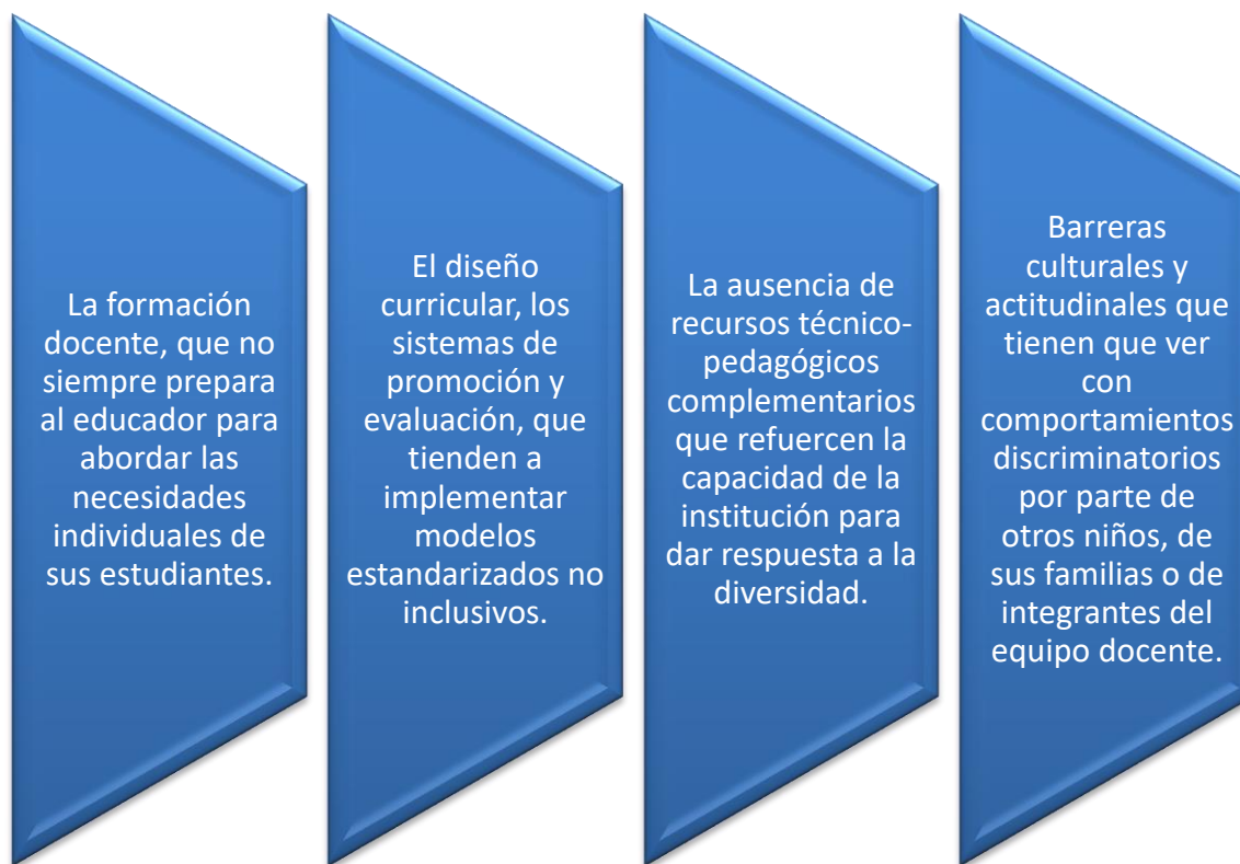
Fig. 1 Diagrama Conceptual
